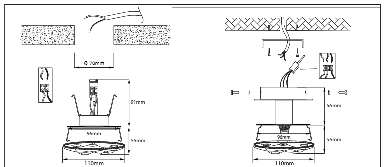
Einbau/recessed
