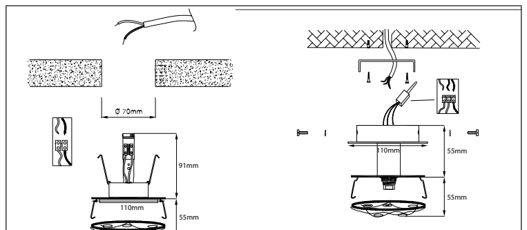
Einbau/recessed
